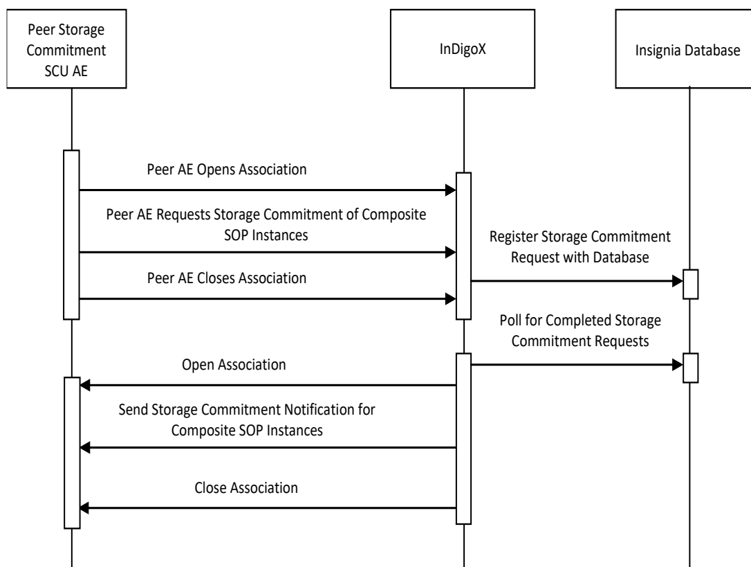
Figure 4.2-1. Sequencing of Activity: Send Commitment Notification over new Association.
