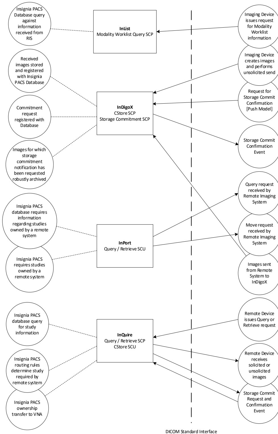
Figure 4.1-1. Insignia PACS DICOM Data Flow Diagram.
